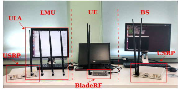
Fig. 1: LTE location system components
