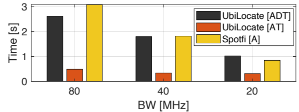
Figure 14: Time complexity for UbiLocate and Spotfi.
