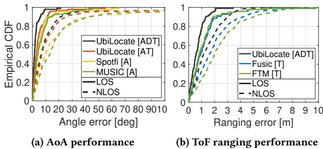
Figure 10: Empirical CDF for AoA and ToF error for all APs, and for LOS (solid lines) and NLOS (dashed lines).
