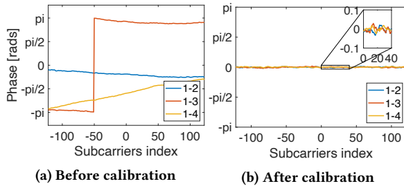
Figure 4: Phase differences for the antennas pairs.
